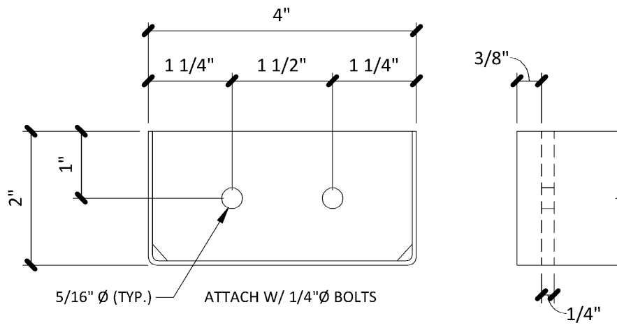
TOP CROSS MEMBER | 09
