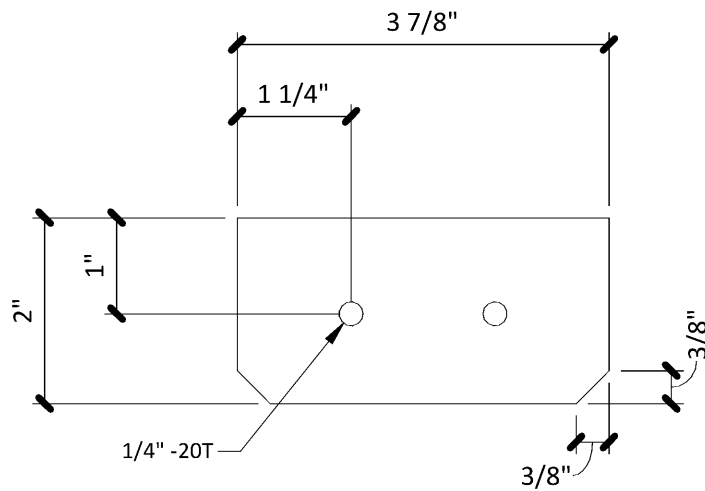
DOUBLE MOUNTING PLATE | 05
