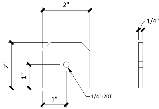
SINGLE MOUNTING PLATE | 04
