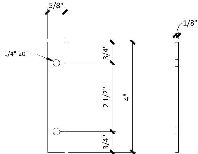
HORIZONTAL BRACE MOUNTING PLATE | 07
