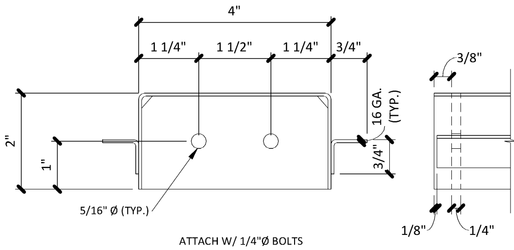
BOTTOM CROSS MEMBER | 03
