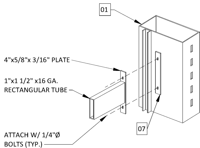
HORIZONTAL BRACE | 08
