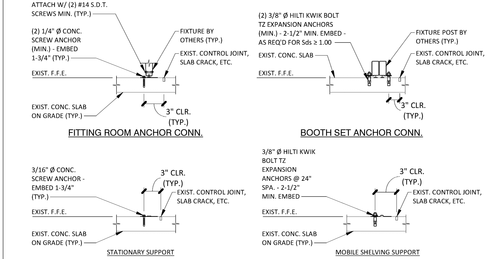
STOARGE RACK ANCHOR CONN.
