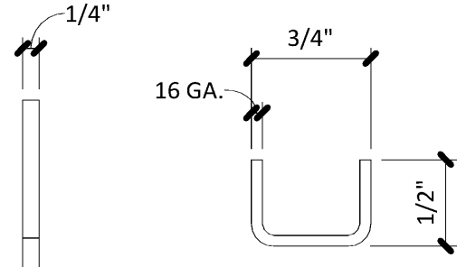
CHANNEL | 06
